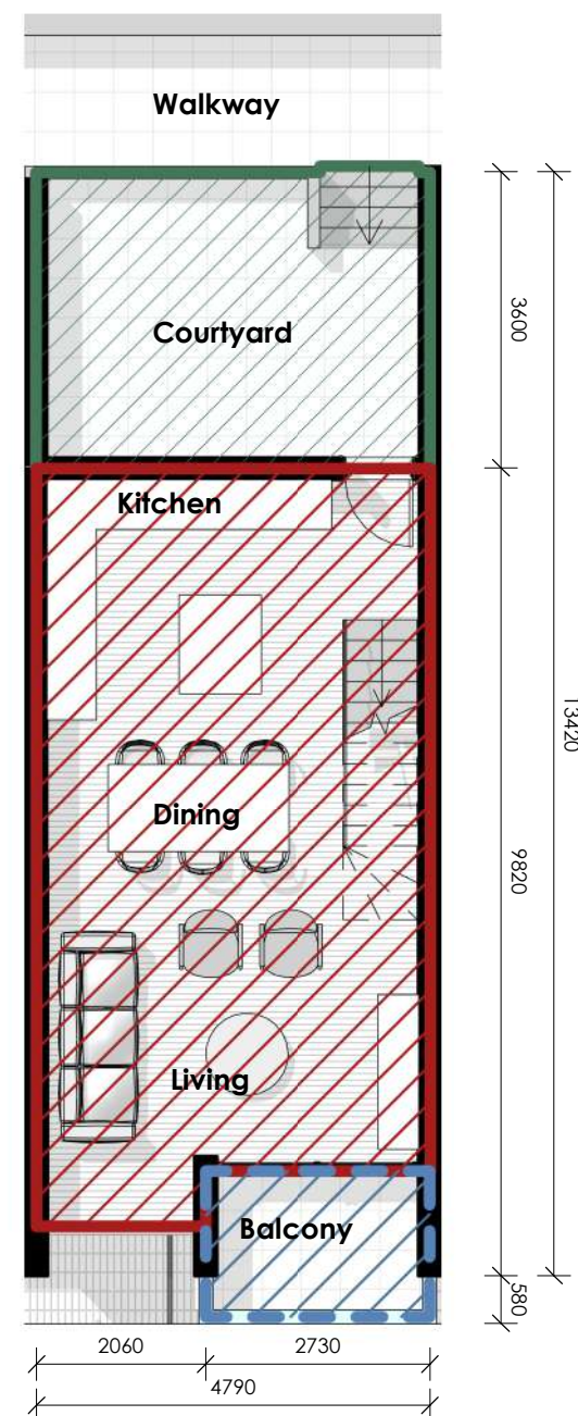
Unit G - 2 Bed 1st Floor 1:100
