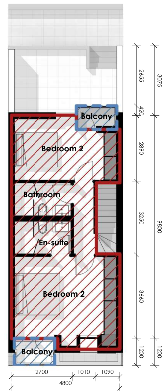
G Unit - 2 Bed 2nd Floor 1:100
