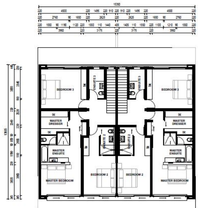
01 - FIRST FLOOR PRESENTATION SCALE 1 : 100
