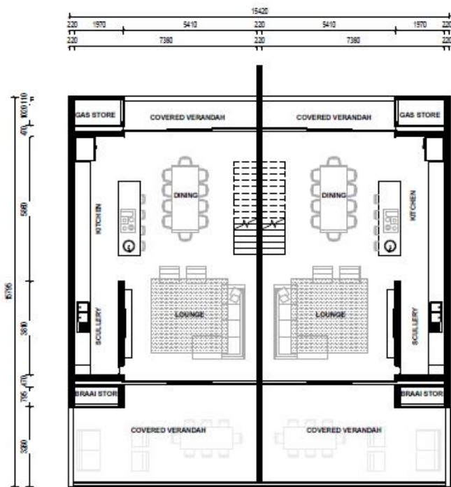
00 - GROUND FLOOR PRESENTATION SCALE 1 : 100
