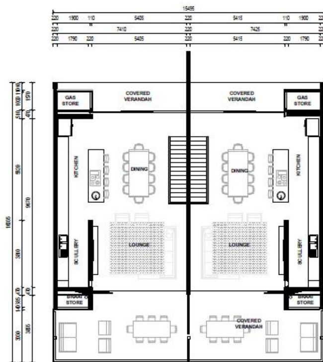
01 - FIRST FLOOR PRESENTATION PLAN SCALE 1 : 100
