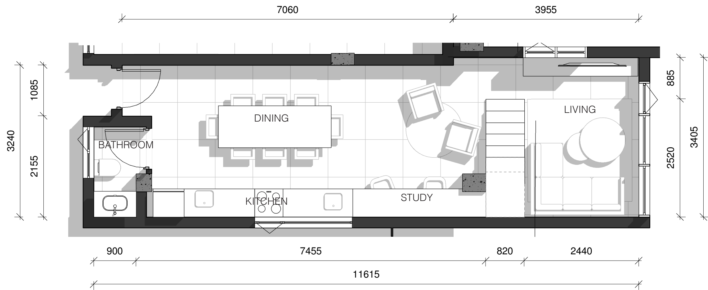
LOFT UNIT _ LEVEL 00
