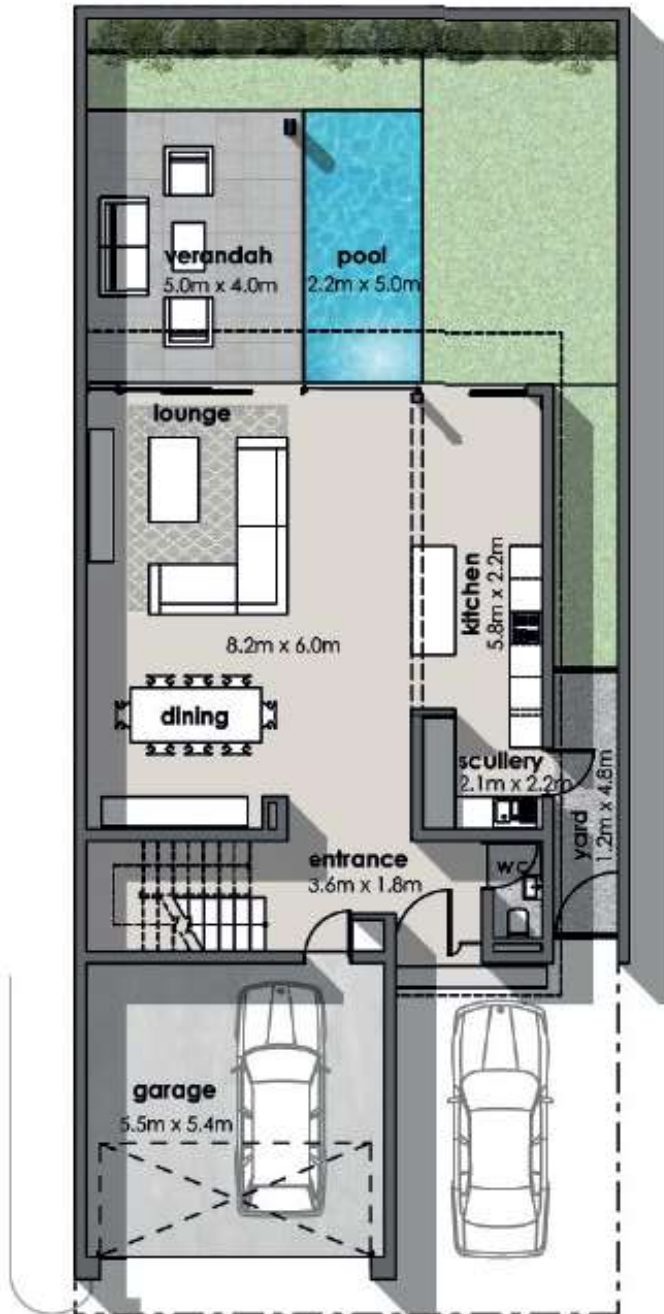
GROUND FLOOR
